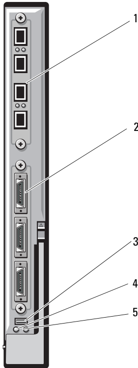
Figure 1-1. PowerConnect M8024 Switch Module
